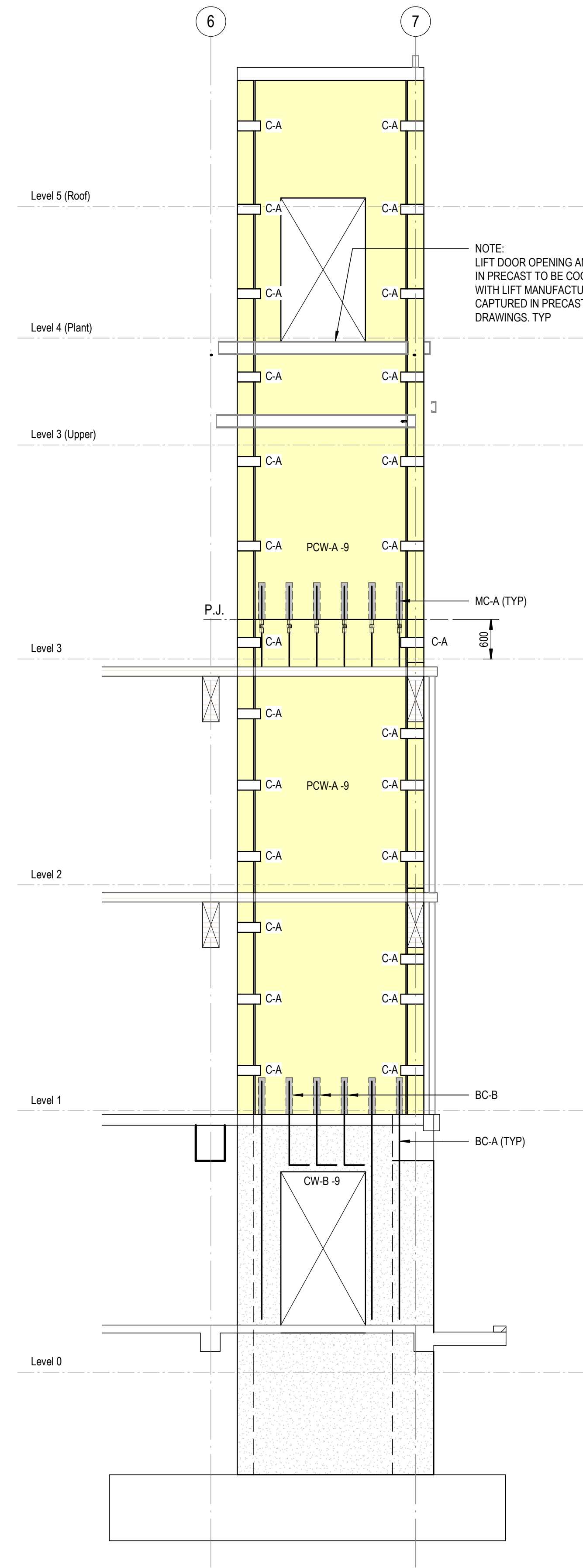
WALL 9 ELEVATION
